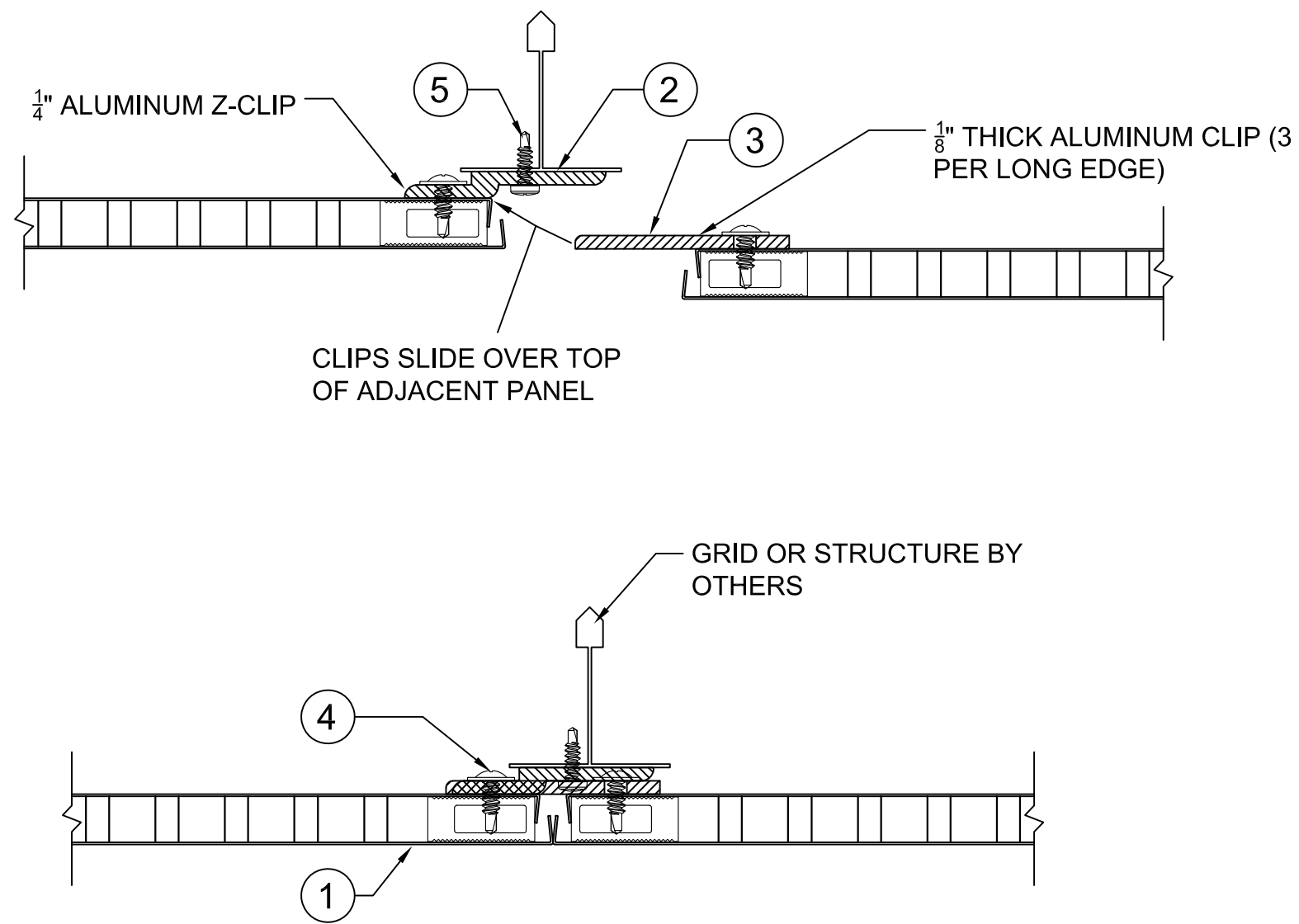
1F CEILING HANGER LINER CEILING
