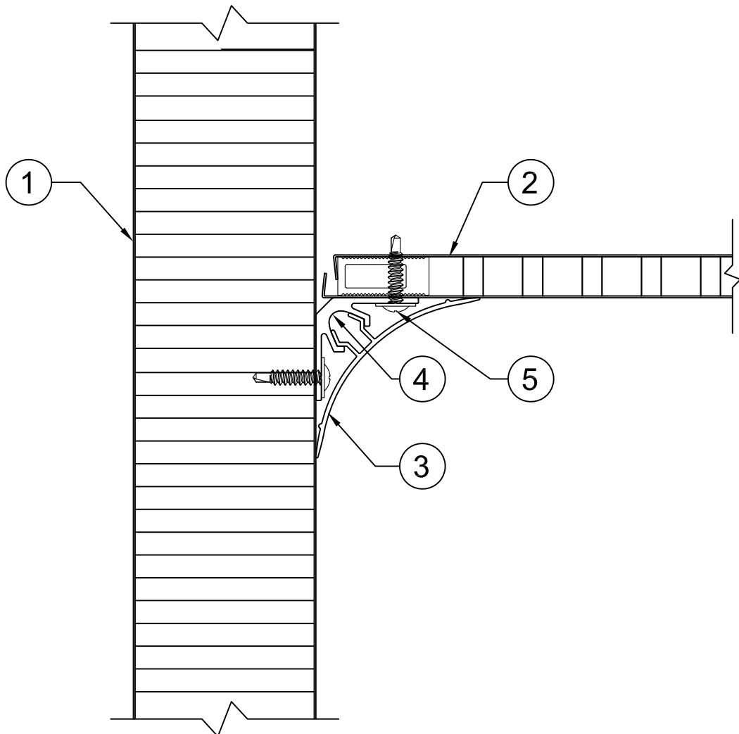
1D WALL TO CEILING 2" STUDLESS WALL
